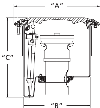
702/703 SLIP-ON BASE
