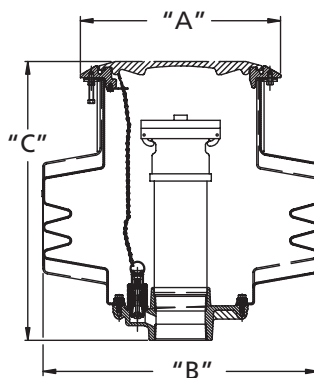
705/715/725 THREADED BASE
