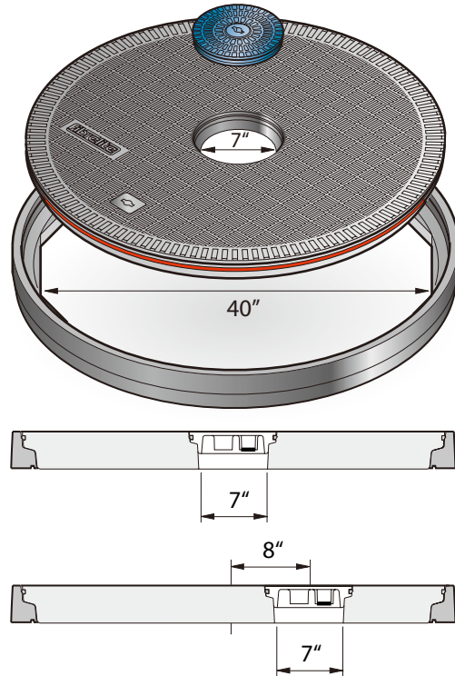
FL100 - 40" dia. Dip Covers
