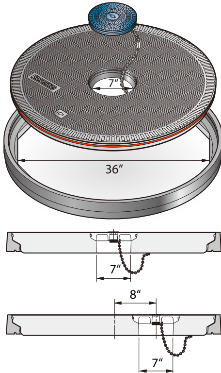
FL90 - 36" dia. Dip Covers
