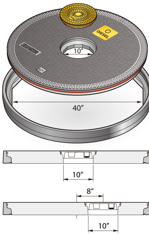
FL100 - 40" dia. Fill Covers
