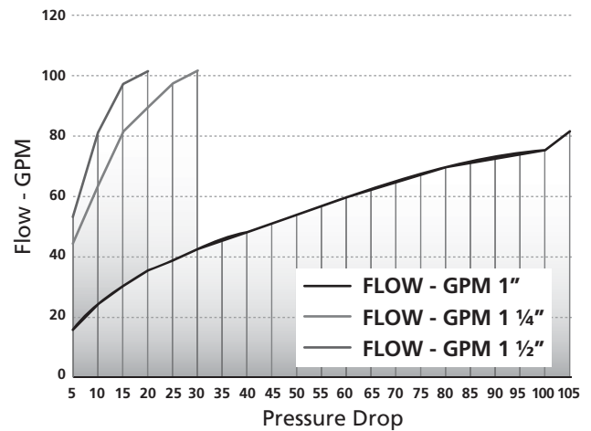
EBW 495 NOZZLES
