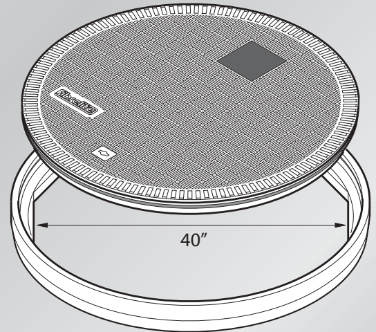
FL100 - 40" dia. flat sealed cover
