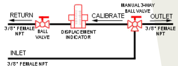
CALIBRATION BLOCK
