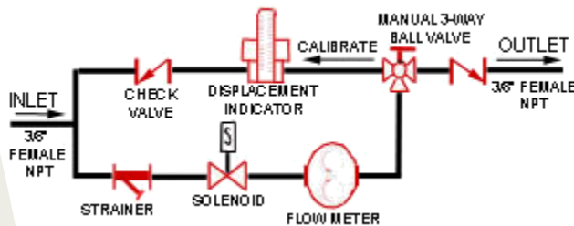
PRECISION CHEMICAL INJECTOR
