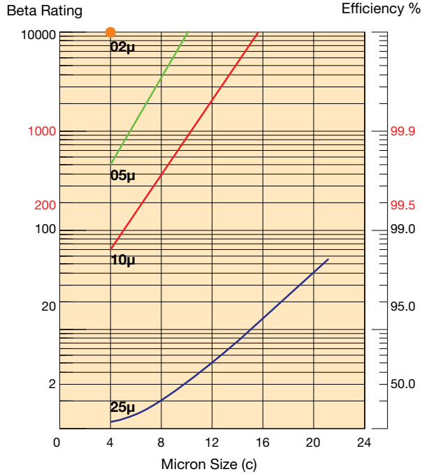
Single-pass tests run per SAE J1985 @ 115 GPM - 5 mg/L BUGL
