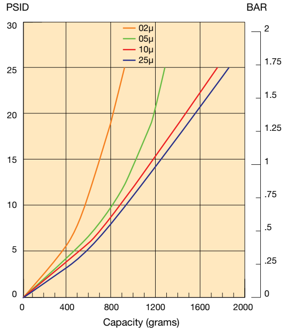
Multi-pass tests run per SAE J905 @ 115 GPM to 25 PSID terminal - 20 mg/L BUGL
