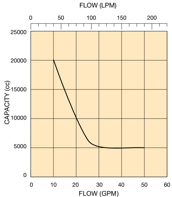
Internal test @ 115 GPM to 25 PSID terminal - 100 ppm H 2 O
