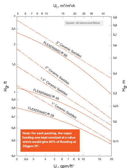
Mass Transfer HTU: FLEXERAMIC® vs. Ceramic Saddles
