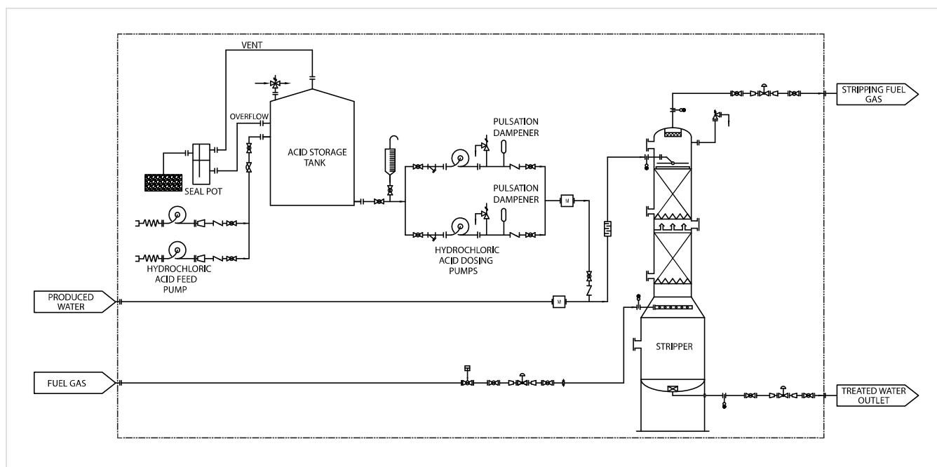
TYPICAL SOUR WATER STRIPPER FLOW SHEET
